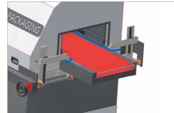
Tunnel con sponde di raffreddamento Refrigerated water cooled guides in tunnel
